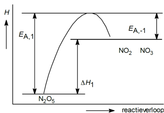
Figuur 49: Experimentele activeringsenergie
